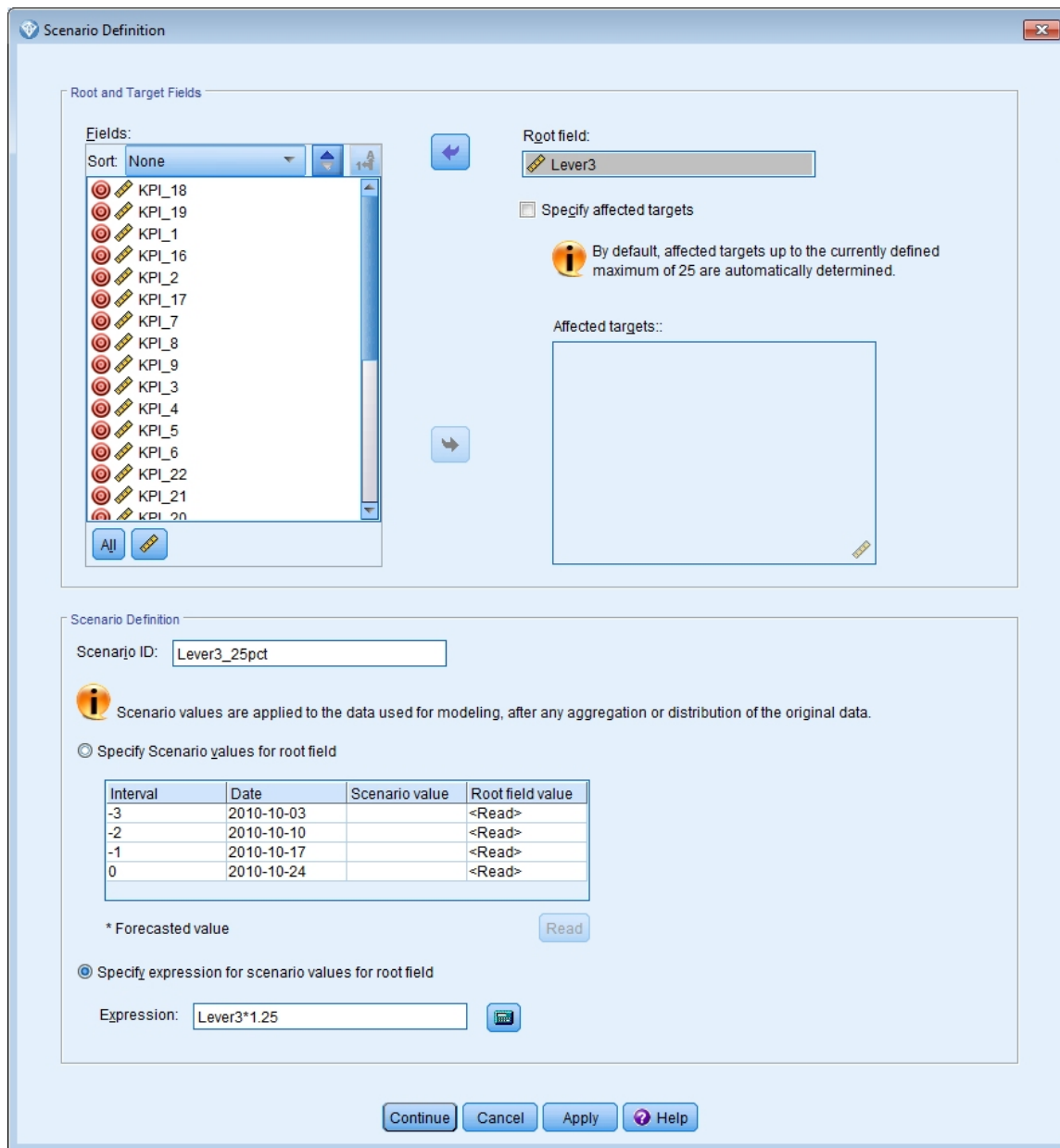
Figure 410. Scenario Definition
