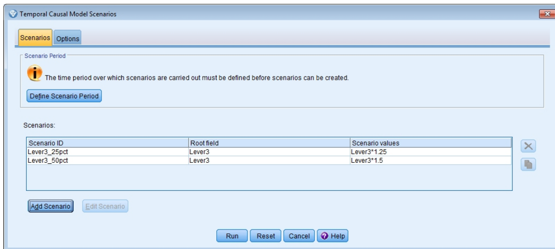
Figure 411. Scenarios
