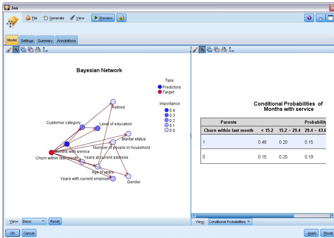
Figure 251. Bayesian Network model showing conditional probabilities
