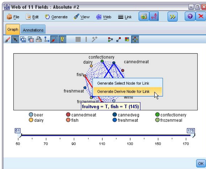
Figure 385. Deriving a flag for each customer group
