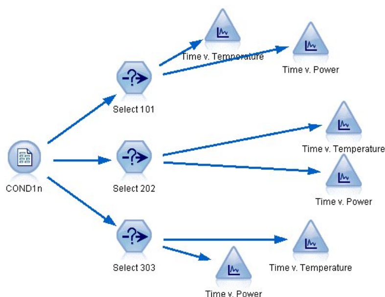
Figure 260. Condplot stream
